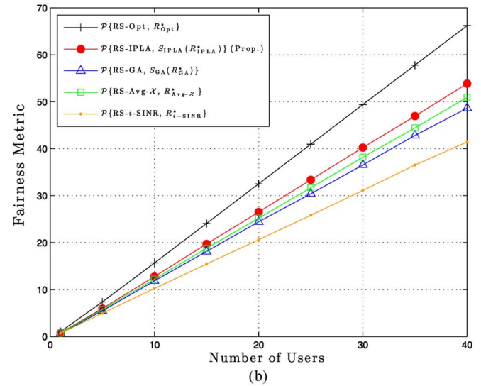
Fig. 5. System performance in an asymmetric user distribution scenario. (a) System DLT versus number of users; (b) fairness metric versus number of users ( K = 6 , r \in [150, 200, 250, 300, 400] m, \theta = \text{Uniform}[-\pi, \pi] , \alpha = 3 , and N_{\max} = 4 ).
