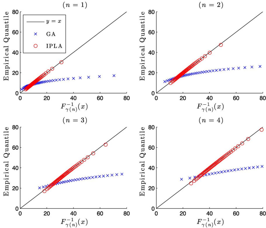
Fig. 2. Q-Q plots of the proposed IPLA and the conventional GA ( K = 6, r = 250 \text{ m}, \theta = \pi/2, \alpha = 3, |w_{u_0}^{(0)}|^2 = 1 , and N_{\max} = 4 ).
